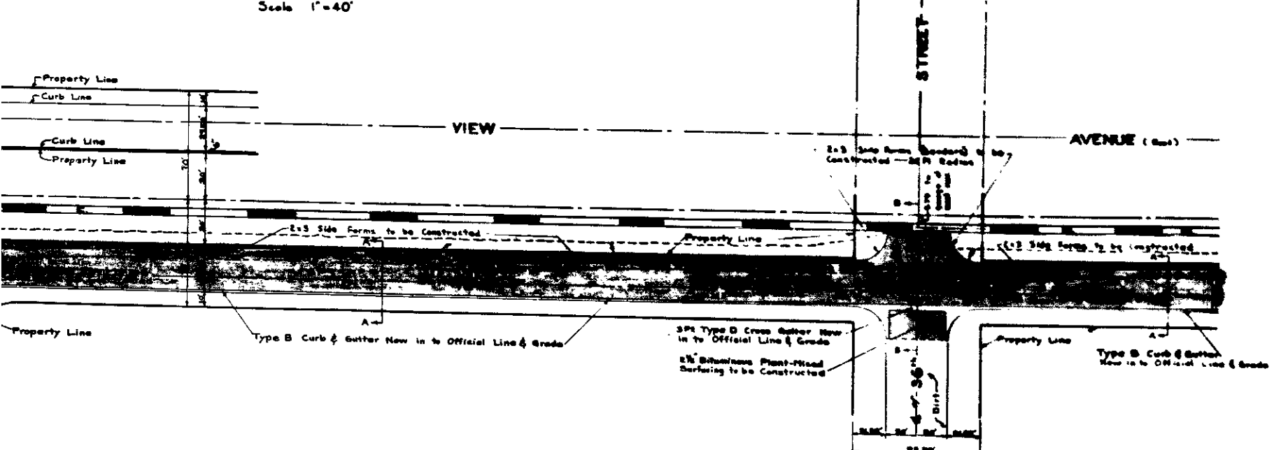
PLAN Scale 1" = 40'
